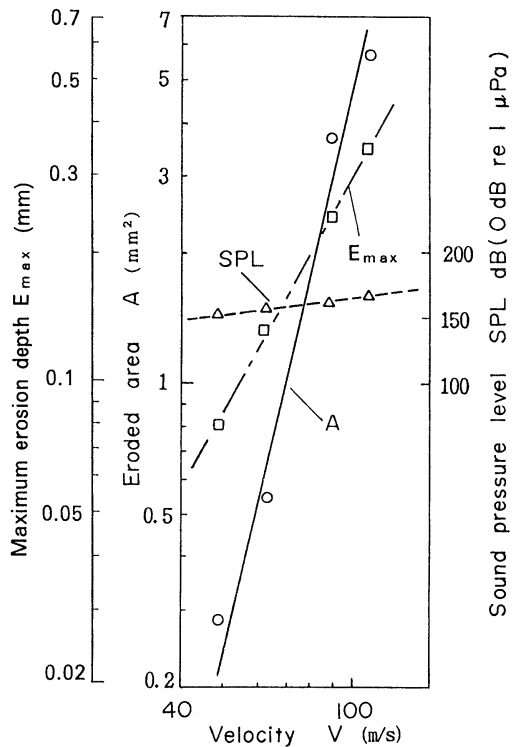
Fig. 6. Correlations of maximum erosion depth E_{max} eroded area A and cavitation noise SPL with velocity V in case of \sigma = 0.25, t = 60 min.
