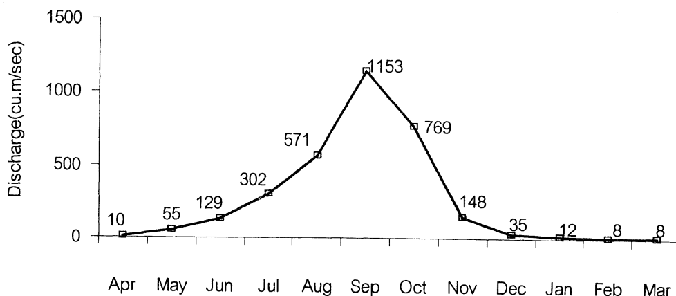
Fig. 6. Monthly discharge of Bangpakong River at the river mouth averaged over the water years 1993-1996.
